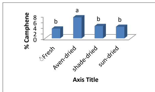
Fig. 4. Comparison of Camphene fresh sample and dry samples of the drying methods. (Significant different at p < 0.05 have been indicated with different letters.)
